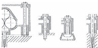
Fixing possibilities
